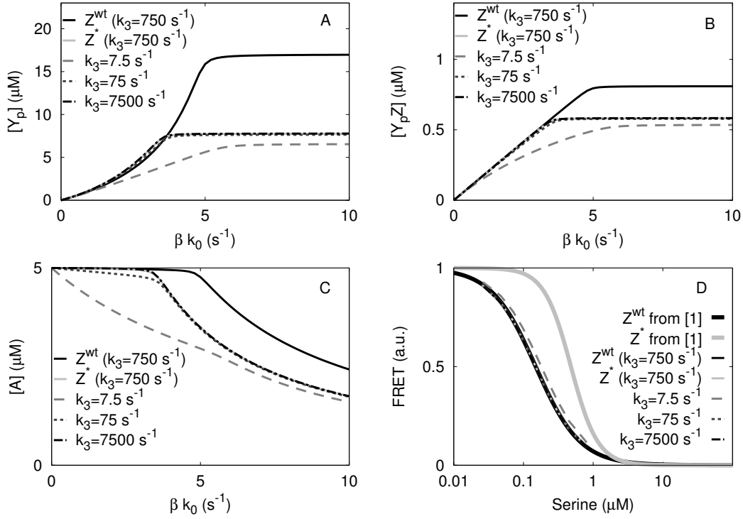
FIGURE 3.6 Effect of k_3 on the response of the commonly adopted chemotaxis model (Equations 3.1-3.3). Shown are the response of [Y_p] (A), [Y_pZ] (B), [A] (C) to changes in the activity of the receptor cluster \beta k_0 and the FRET signal as a function of serine concentration (D). The baseline parameters are given in Fig. 3.5.
