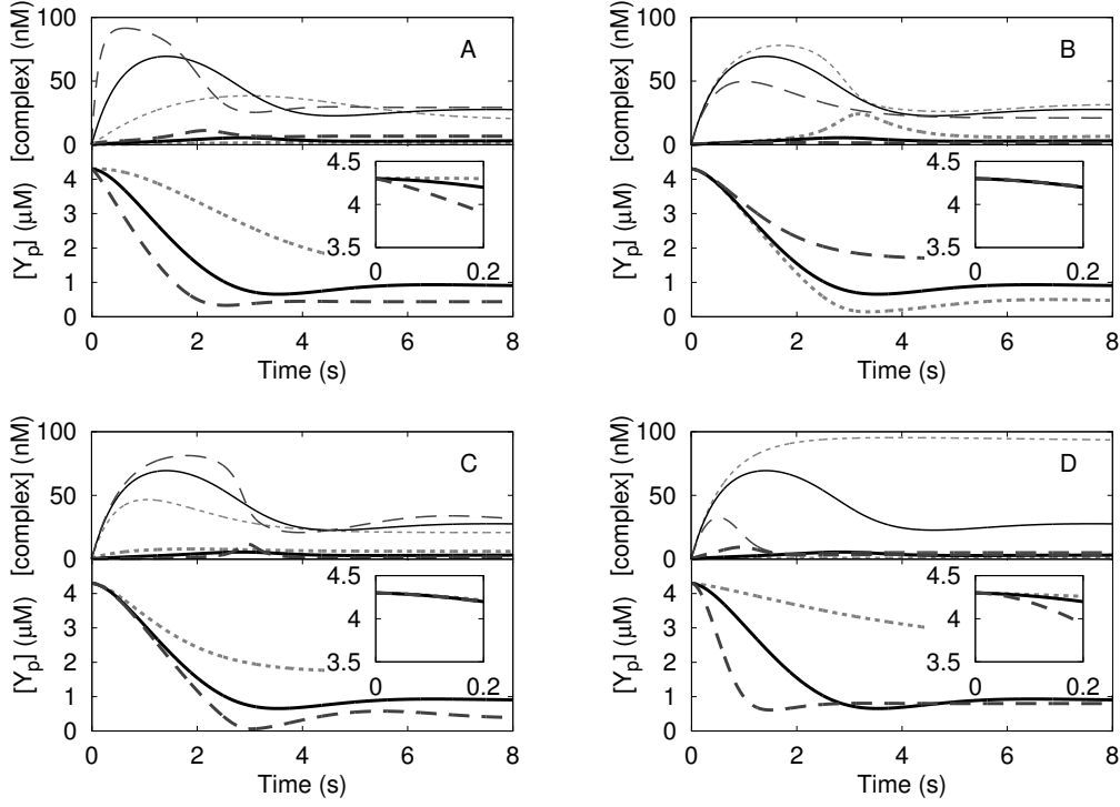
FIGURE 4.5 Effect of varying the parameters of the cooperative model (Equations 4.10–4.11) on the phosphatase kinetics. The upper panels show the concentrations of [(Y_p)_2Z] (upper three curves) and of [Y_pZ] (lower three curves) as functions of time. The lower panels show the evolution of the concentration of CheY_p upon addition of CheZ . The concentration of CheY_p does not go to zero because CheY is continuously phosphorylated by AcP , as in the experimental setup [76]. The insets show a magnification of the initial delay. A. Effect of k_4 . B. Effect of k_6 . C. Effect of k_{10} . D. Effect of k_{12} . The parameter values are 0.2 (dotted), 1 (solid) and 5 (dashed) times the baseline parameters of Fig. 4.7.
