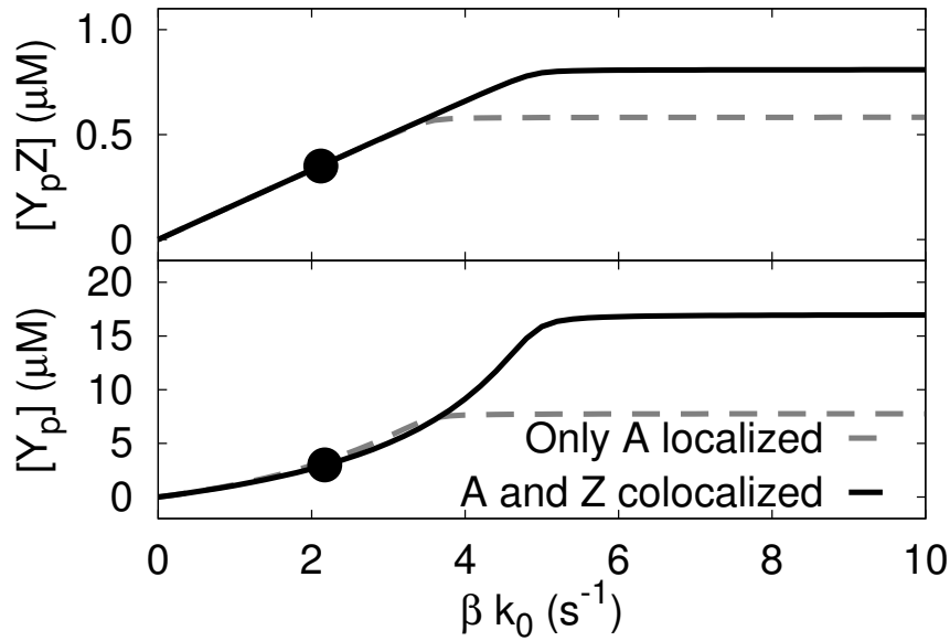
FIGURE 3.4 Total, integrated concentration of \text{CheY}_p\text{CheZ} , \int_0^L dx[\text{Y}_p\text{Z}](x) , and \text{CheY}_p , \int_0^L dx[\text{Y}_p](x)dx , as a function of \beta k_0 for the canonical model of the chemotaxis network of E. coli , shown in Equations 3.1-3.3. The solid curves correspond to wild-type cells in which CheA and CheZ are colocalized at the receptor cluster, while the dashed curves correspond to the mutant cells in which CheA is localized at the pole, while CheZ freely diffuses in the cytoplasm. The bullets correspond to the adapted state of the system. The diffusion constant of the diffusing components is D = 5\mu\text{m}^2\text{s}^{-1} [71]. For other parameter values, see [45].
